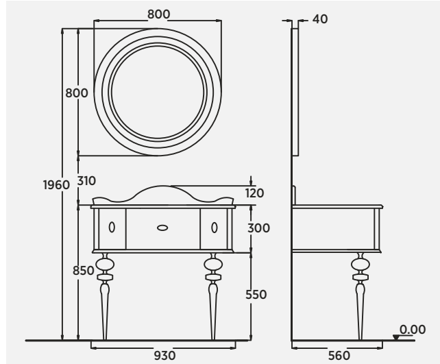
Charlotte 95 cm Lavabo Dolabi | Washbasin Cabinet | Mobile Lavabo Charlotte 80 cm Aydınlatmalı Ayna | Illuminated Mirror | Specchio Illuminato
