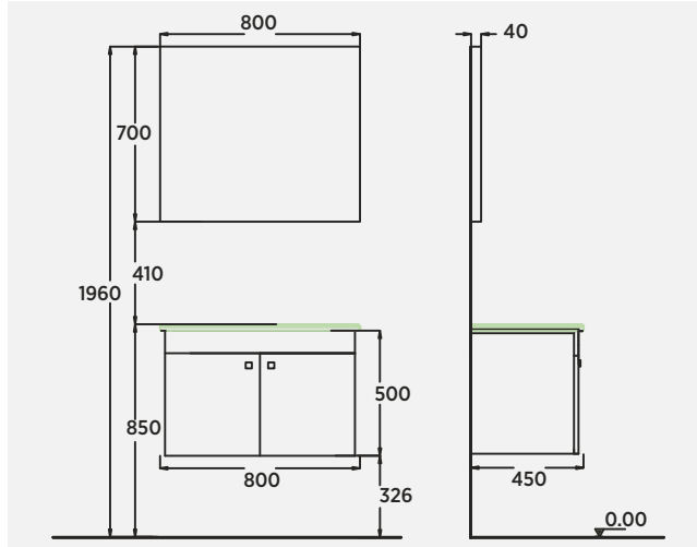
Luna 80 cm Lavabo Dolabı Washbasin Cabinet | Mobile Lavabo Luna 80 cm Ortak Ayna Mirror | Specchio
