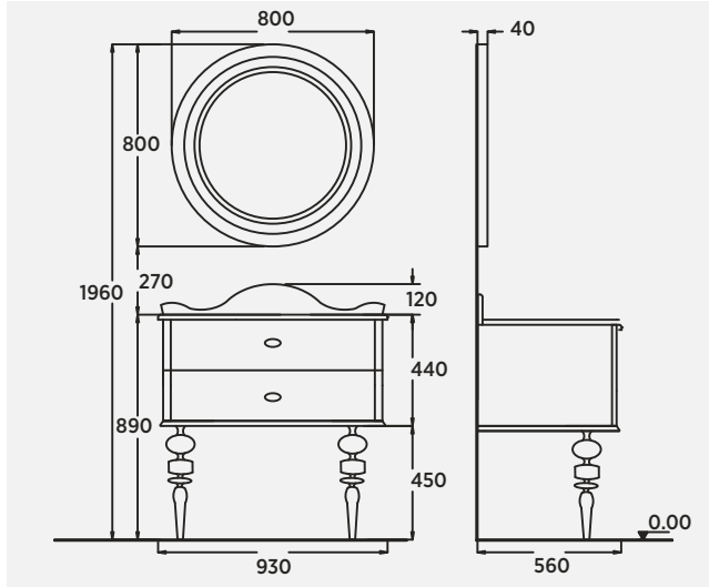
Charlotte Queen 95 cm Lavabo Dolabı Washbasin Cabinet | Mobile Lavabo Charlotte Queen 80 cm Aydınlatmalı Ayna Illuminated Mirror | Specchio Illuminato
