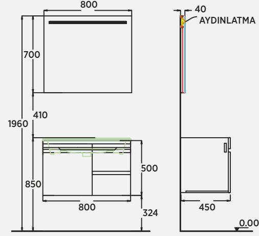
Vico Duo 80 cm Lavabo Dolabi Washbasin Cabinet | Mobile Lavabo Vico Duo 80 cm Aydınlatmalı Ayna Illuminated Mirror | Specchio Illuminato
