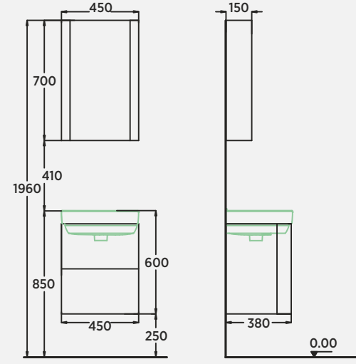
Bold 45 cm Lavabo Dolabı Washbasin Cabinet | Mobile Lavabo
