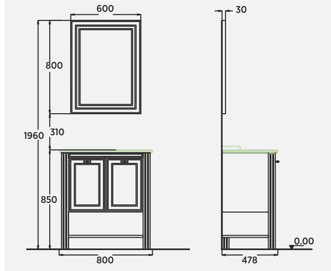
Greta 80 cm Lavabo Dolabı | Washbasin Cabinet | Mobile Lavabo Greta 60 cm Ayna | Mirror | Specchio
