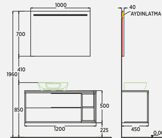
Allure 120 cm Lavabo Dolabı Washbasin Cabinet | Mobile Lavabo Ortak 120 cm Aydınlatmalı Ayna Illuminated Mirror | Specchio Illuminato
