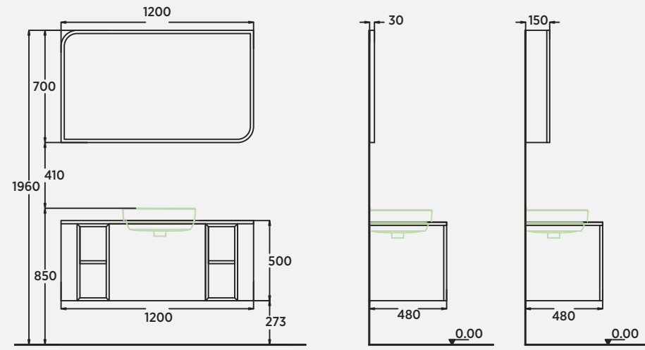
Drexel 120 cm Lavabo Dolabi | Washbasin Cabinet | Mobile Lavabo
