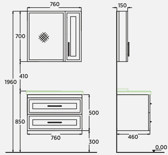
Victorian 80 cm Lavabo Dolabı Washbasin Cabinet | Mobile Lavabo Victorian 80 cm Aydınlatmalı Ayna Illuminated Mirror | Specchio Illuminato
