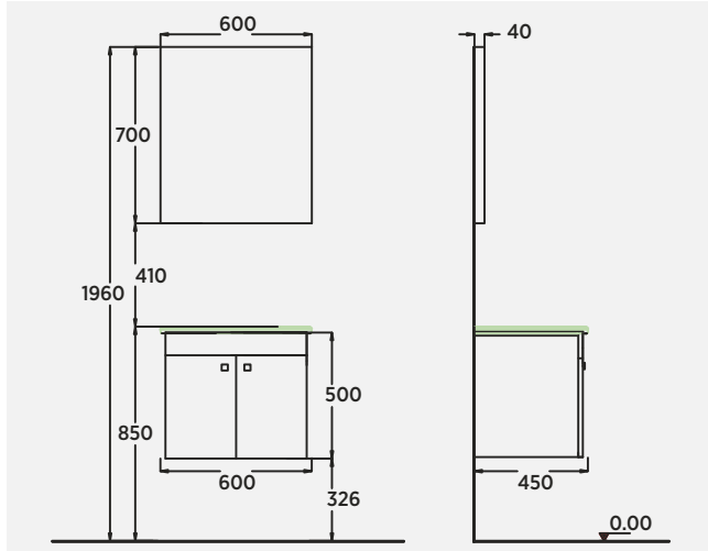
Luna 60 cm Lavabo Dolabı Washbasin Cabinet | Mobile Lavabo Luna 60 cm Ortak Ayna Mirror | Specchio
