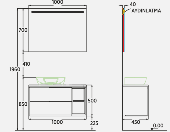
Allure 100 cm Lavabo Dolabı Washbasin Cabinet | Mobile Lavabo Ortak 100 cm Aydınlatmalı Ayna Illuminated Mirror | Specchio Illuminato
