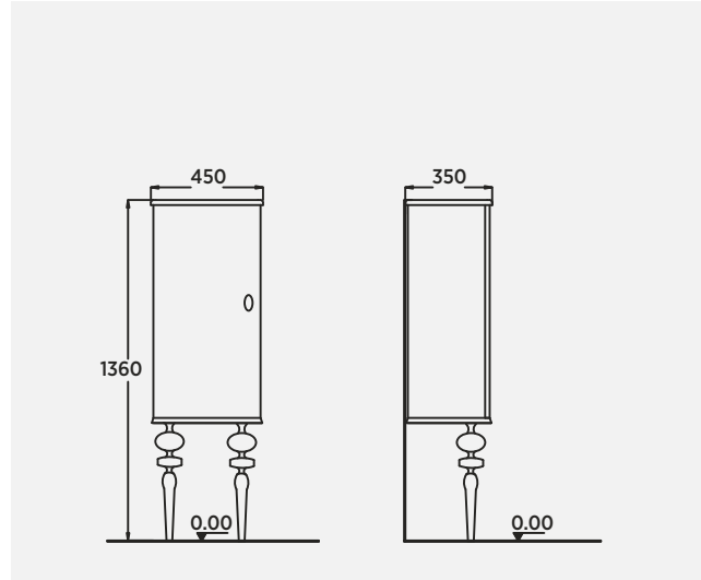
Charlotte 45 cm Boy Dolabi | Tall Cabinet | Armadio Alto
