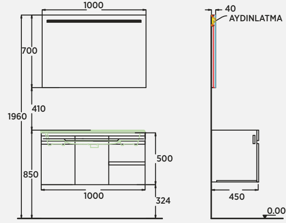
Vico Duo 100 cm Lavabo Dolabi Washbasin Cabinet | Mobile Lavabo Vico Duo 100 cm Aydınlatmalı Ayna Illuminated Mirror | Specchio Illuminato
